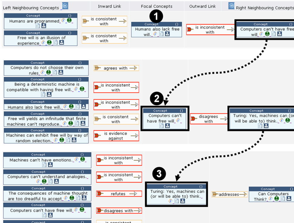
Figure 9: Navigating the 'Neighbourhood' around a concept. Clicking on a concept makes it the central node, and displays the incoming and outgoing links one step away (We gratefully acknowledge Robert Horn's paper maps as the source for this example: www.macrovu.com/CCTGeneralInfo.html ).
