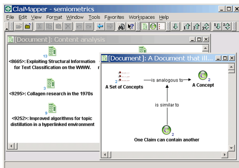
Figure 5: Modelling claims in ClaiMapper. In the left pane is a collection of documents (the digit on each icon indicates how many concepts are annotated on it). Double-clicking one of these opens a new window, e.g. on the right, showing two Concepts, a Set and two Claim triples, one of which is the right-hand side of the other
