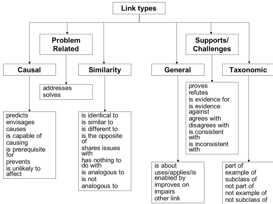
Figure 2: Taxonomy of rhetorical link types
